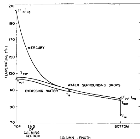
Fig. 7. Probable temperature profiles in column.
